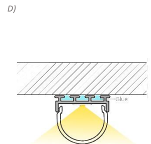
C); D) Application example – Other ways of mounting [C) screw; D) glue]
