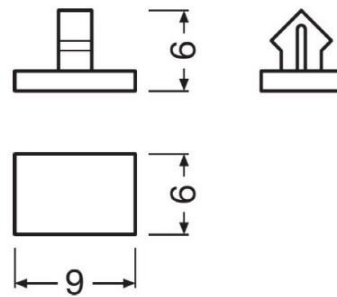
Plastic Clip for combining track and mounting profile FX-QMW-G1-XCLPL1-DIV1 Order code 4052899446731
