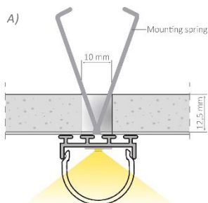
A); B) Application example – Drywall [A) metal spring; B) mounting profile]
