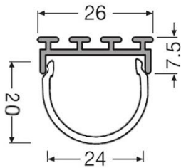
Wide Track + Wide cover round frosted matte FX-QMW-G1-CRD-300
