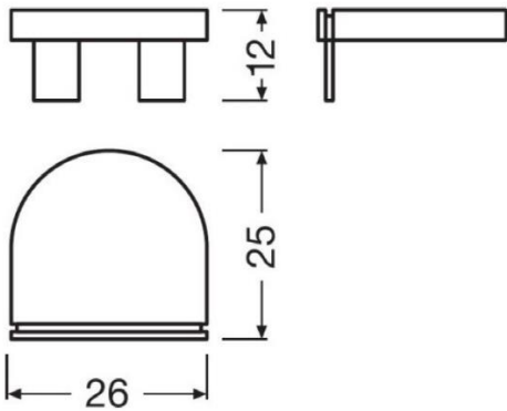
Plastic Round end cap grey plain FX-QMW-G1-ERGP-TU26H8 Order code 4052899450271
