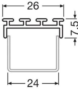
Wide Track FX-QMW-G1-TU26H8-300 Order code 4052899448643
