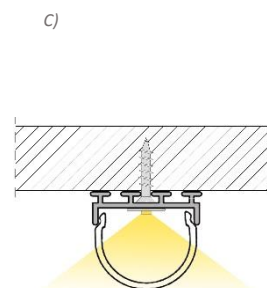
C); D) Application example – Other ways of mounting [C) screw; D) glue]
