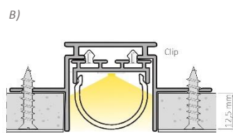
Wide track + Wide cover round frosted matte
